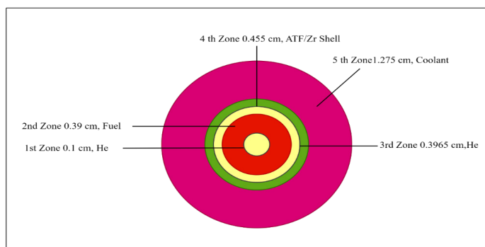
Figure 1. Fuel rod including ATF cladding materials
