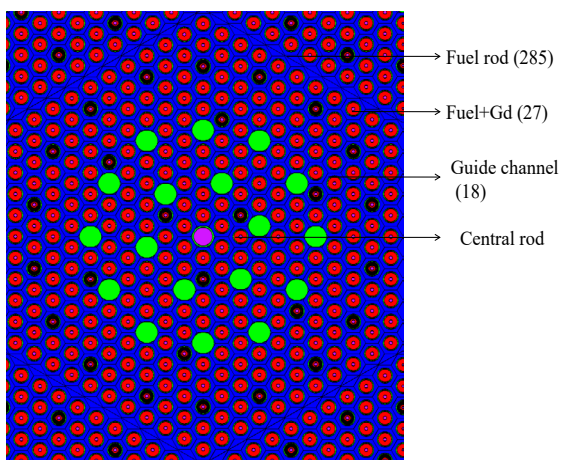
Figure 2. Fuel Assembly
