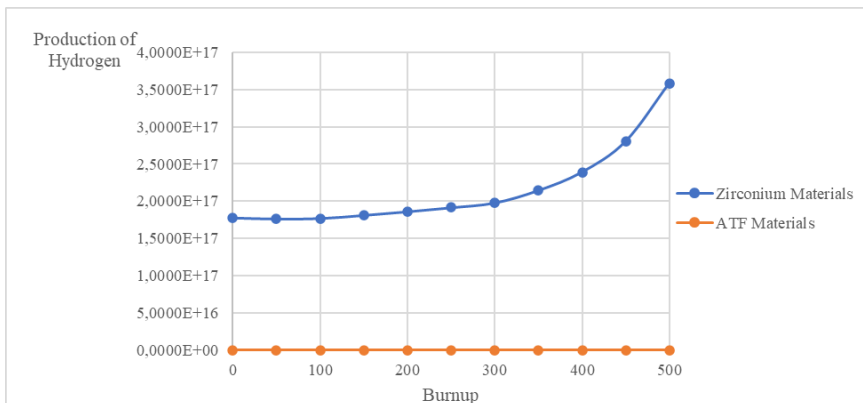
Figure 3. Hydrogen production vs burnup for Zn and AFT materials
